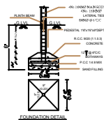
FOUNDATION DETAIL
