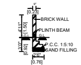
SECTION - CC
