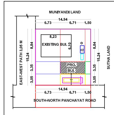
SITE PLAN CUM LOCATION PLAN
