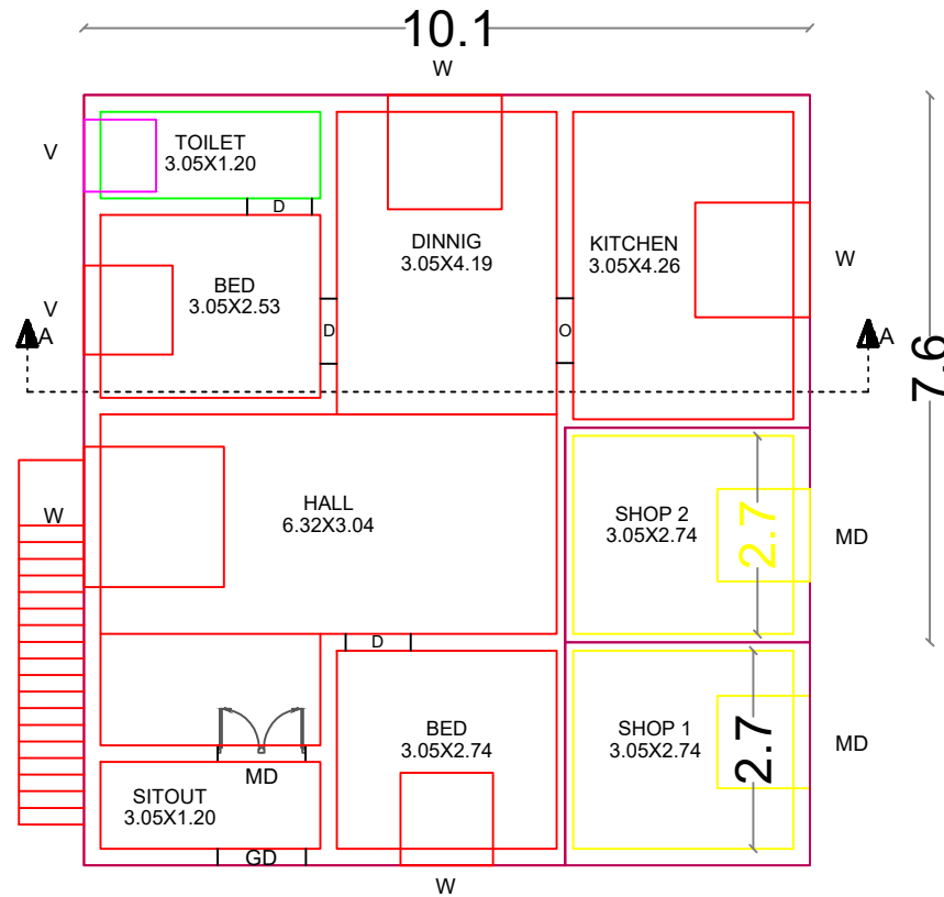
PROPOSED RESIDENTIAL AND COMMERCIAL GROUND FLOOR PLAN
