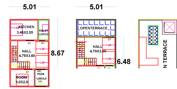
GROUND FLOOR PL
