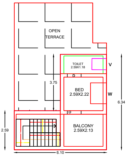
PROPOSED RESIDENTIAL FIRST FLOOR PLAN
