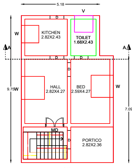
PROPOSED RESIDENTIAL GROUND FLOOR PLAN
