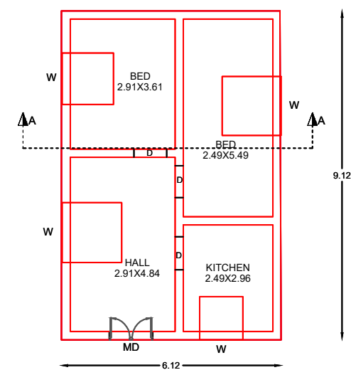
PROPOSED RESIDENTIAL GROUND FLOOR PLAN
