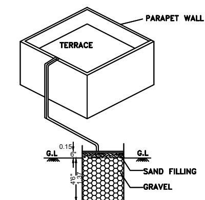
COLLECTION OF SUMP RAINWATER HARVEESTING FROM TERRACE
