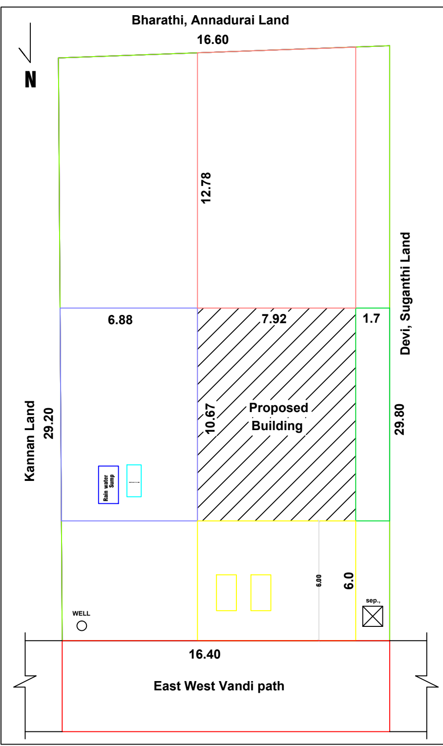
SITE PLAN CUM KEYPLAN
