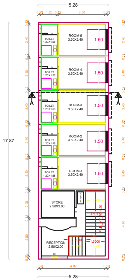
GROUND FLOOR PLAN PROPOSED
