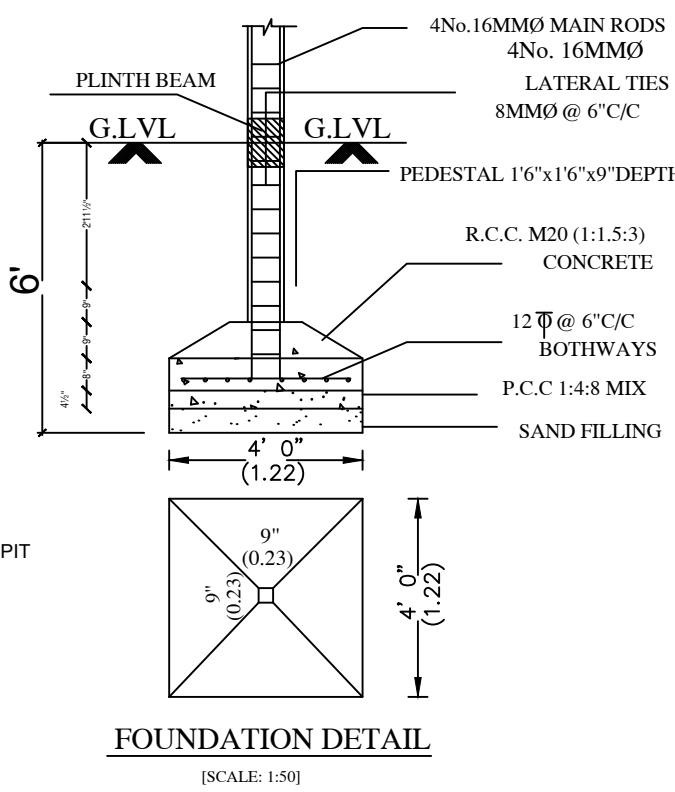
FOUNDATION DETAIL
