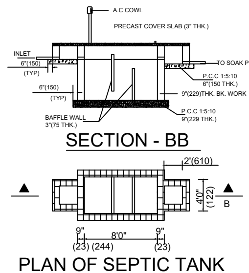
PLAN OF SEPTIC TANK
