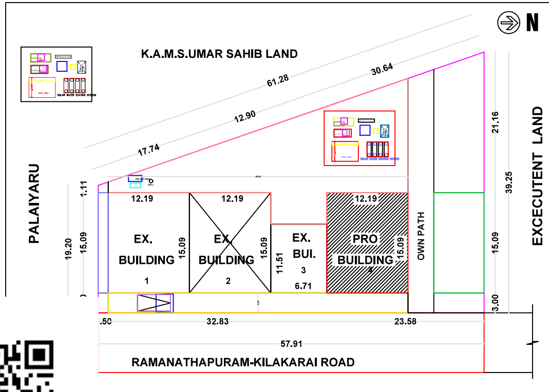
SITE PLAN & LOCATION PLAN
