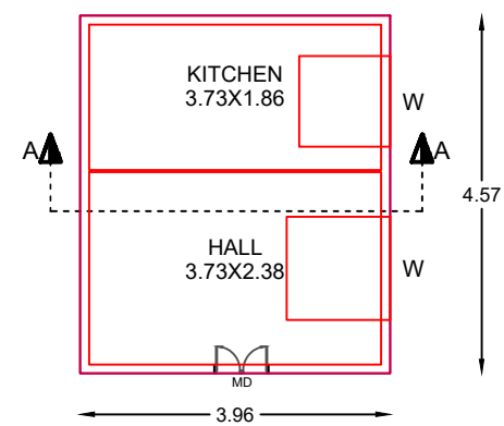
PROPOSED RESIDENTIAL GROUND FLOOR PLAN
