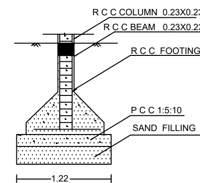
FOUNDATION DETAILS
