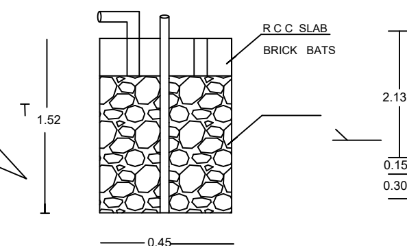
Percolation Pit
