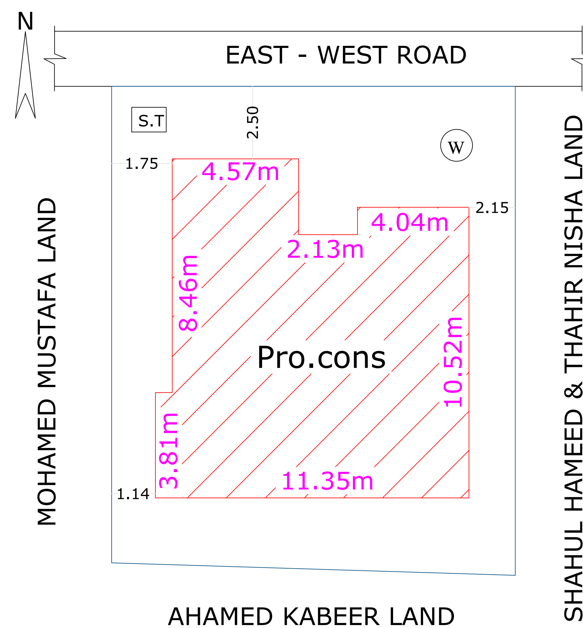
SITE PLAN
