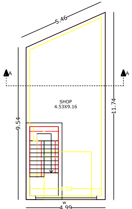
PROPOSED COMMERCIAL SECOND FLOOR PLAN
