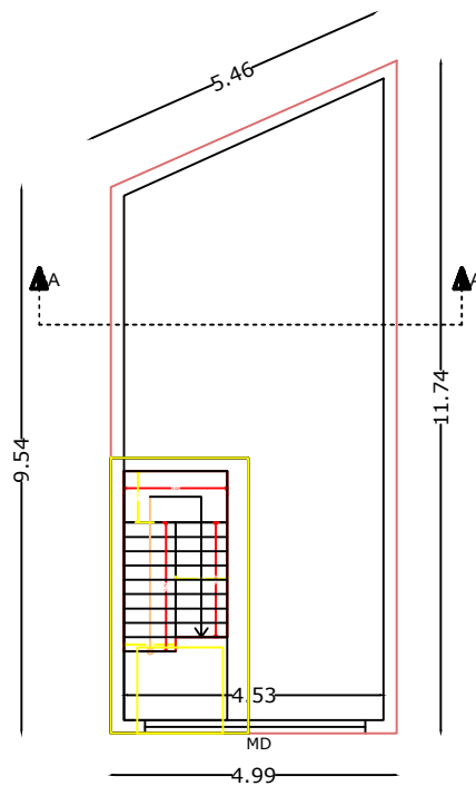
PROPOSED COMMERCIAL STILT FLOOR PLAN
