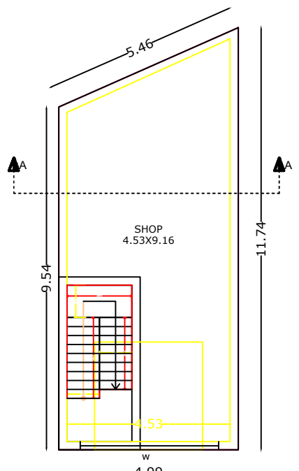
PROPOSED COMMERCIAL FIRST FLOOR PLAN
