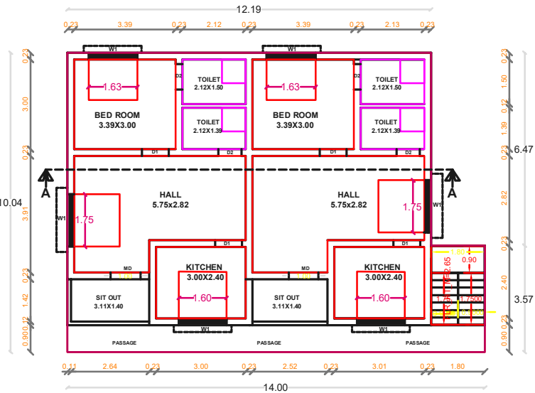
FIRST FLOOR PLAN PROPOSED
