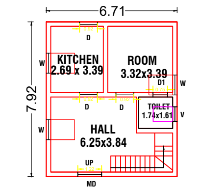
PRO., GROUND FLOOR PLAN
