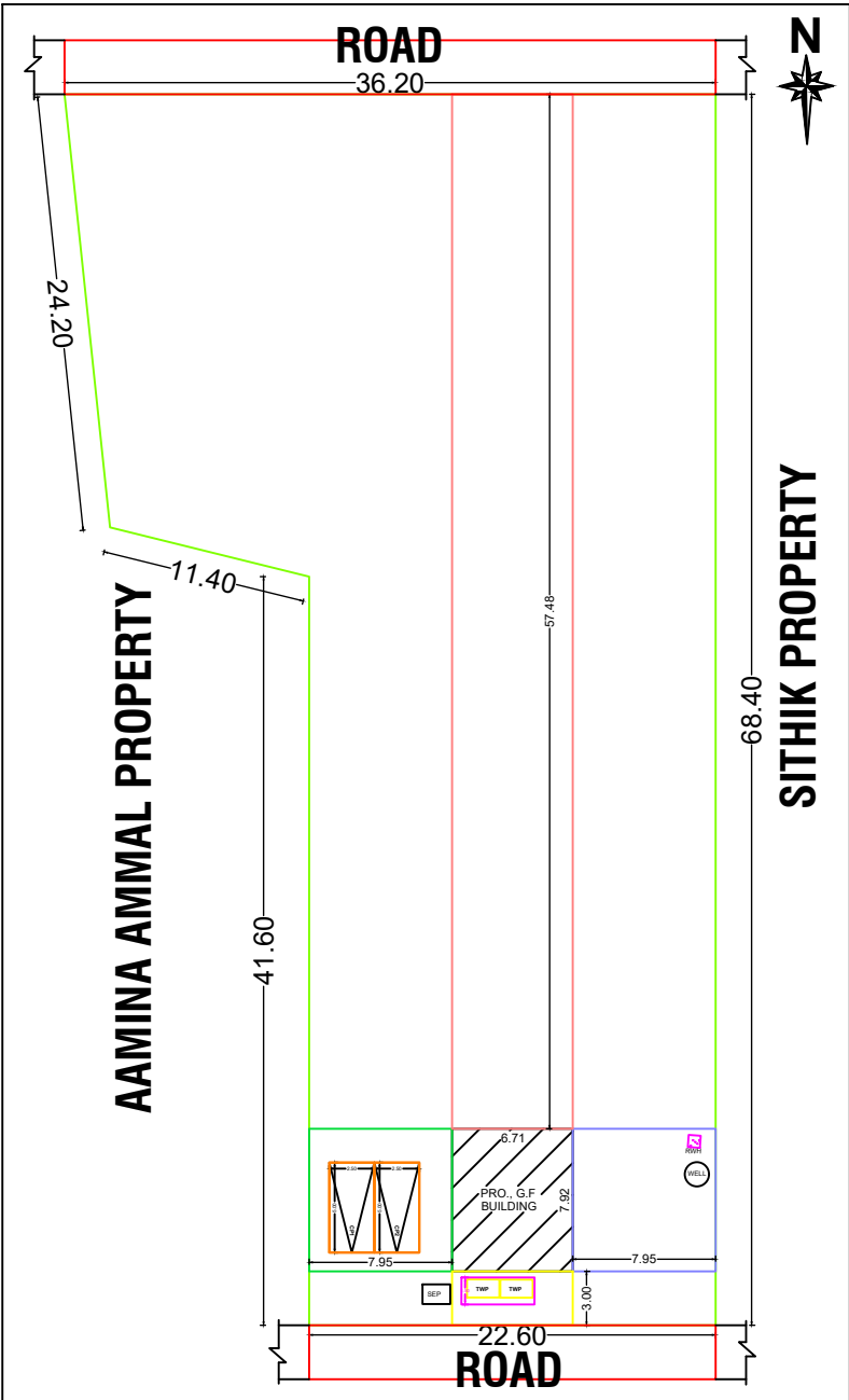
SITE PLAN
