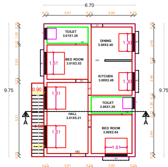
GROUND FLOOR PLAN PROPOSED
