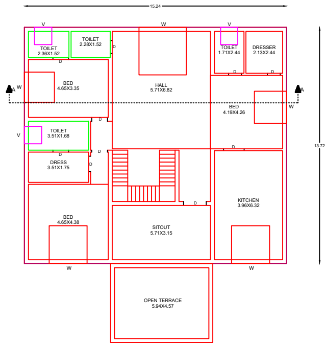
PROPOSED RESIDENTIAL FIRST FLOOR PLAN
