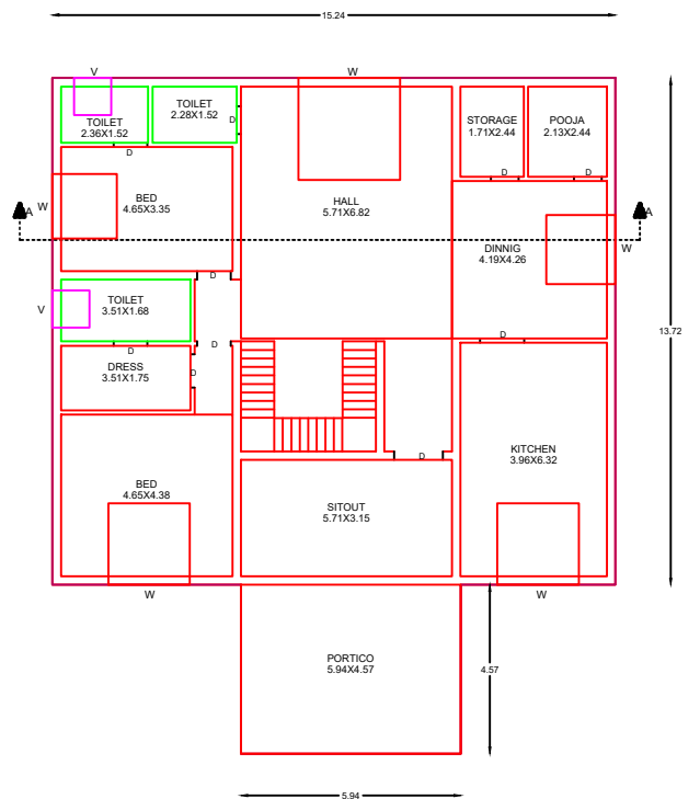
PROPOSED RESIDENTIAL GROUND FLOOR PLAN
