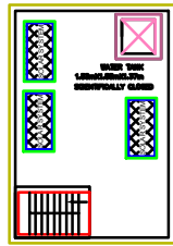
TERRACE FLOOR PLAN
