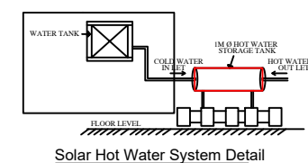
Solar Hot Water System Detail
