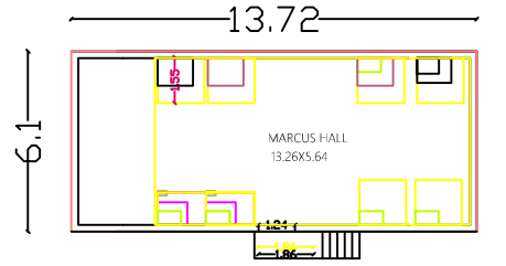
SITE PLAN CUM GROUND FLOOR PLAN
