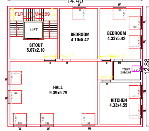
PRO., THIRD FLOOR PLAN
