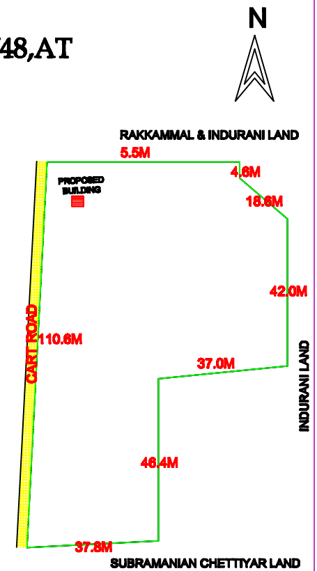
SITE PLAN SCALE NTS
