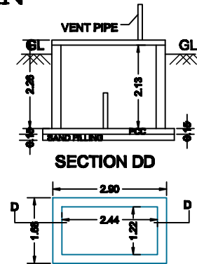
SEPTIC TANK
