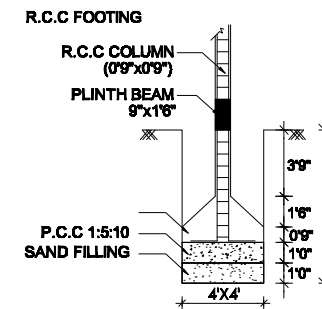
FOUNDATION DETAILS (SCALE 1" = 4'0")
