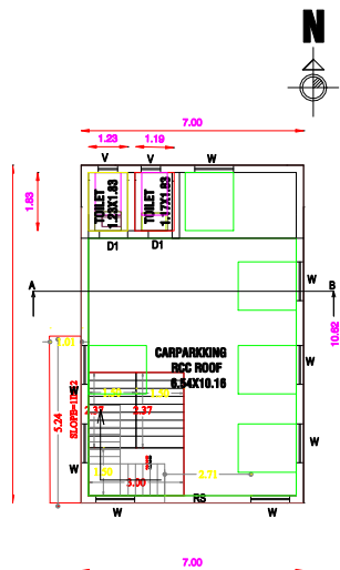
STILT FLOOR PLAN [CAR PARKING]
