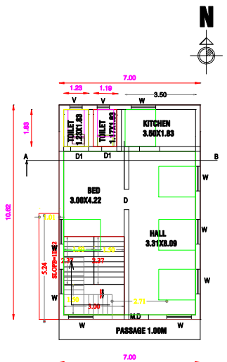
FIRST FLOOR PLAN [DWELLING BUILDING]
