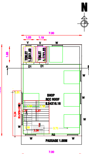
GROUND FLOOR PLAN [SHOP]
