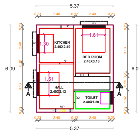
GROUND FLOOR PLAN PROPOSED
