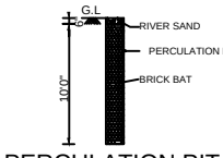
PERCOLATION PIT
