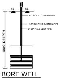
BORE WELL
