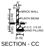
SECTION - CC
