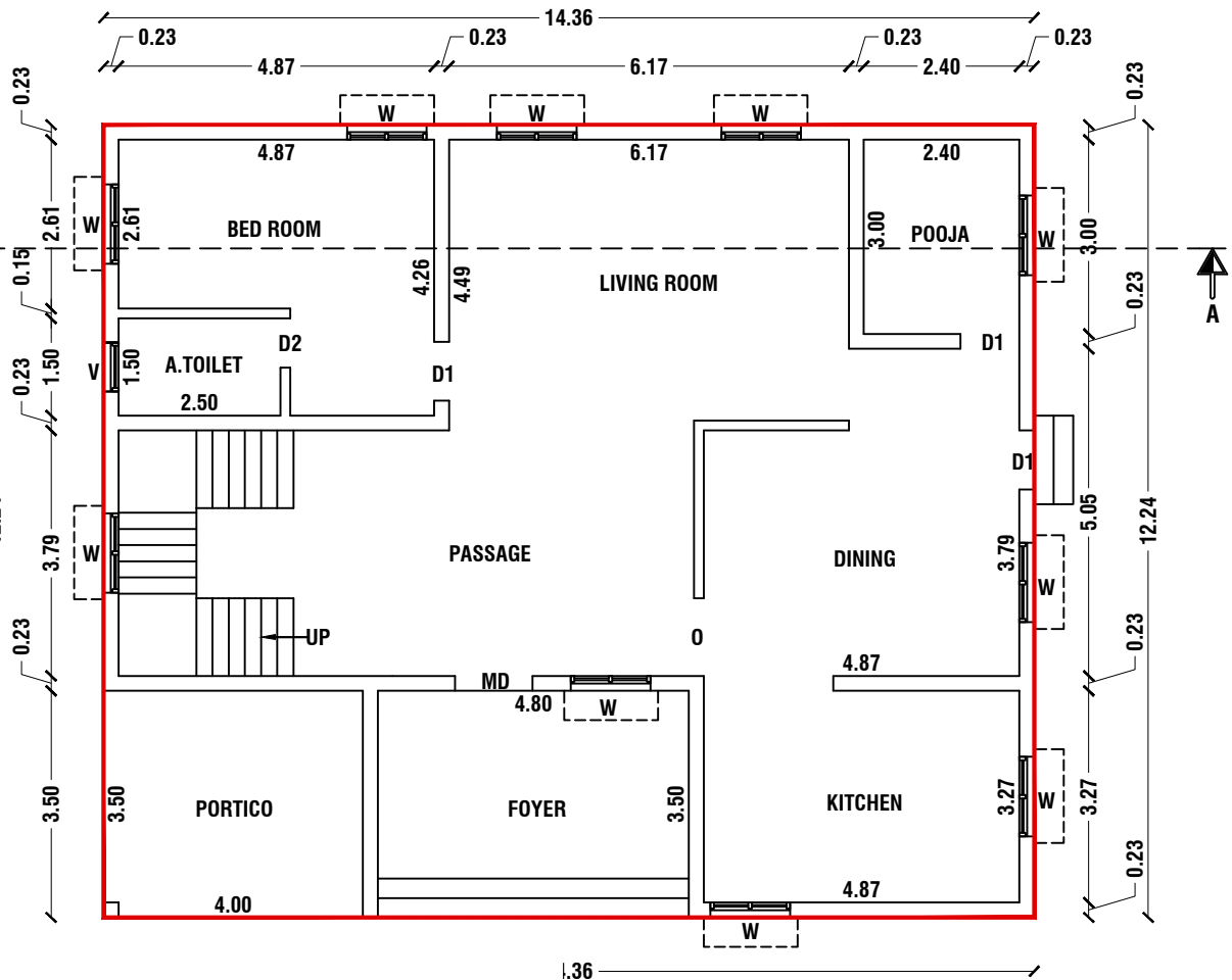
FLOOR PLAN
