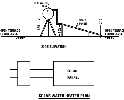
SOLAR WATER HEATER PLAN
