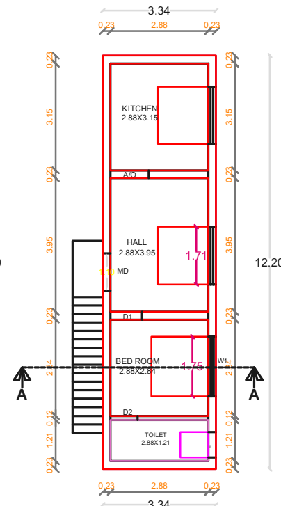
FIRST FLOOR PLAN PROPOSED
