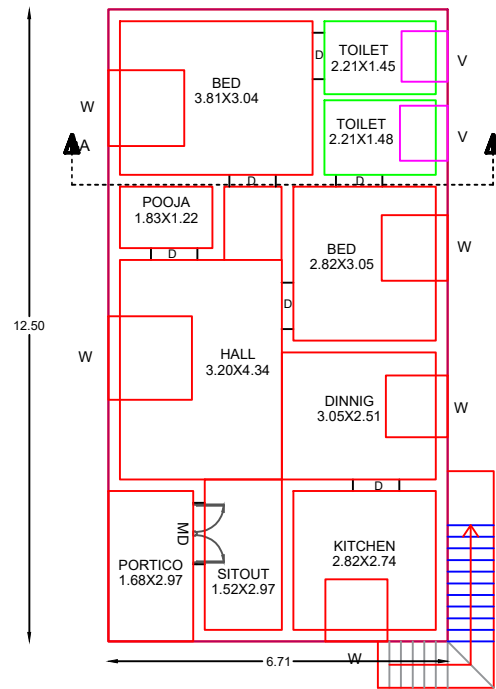
PROPOSED RESIDENTIAL GROUND FLOOR PLAN
