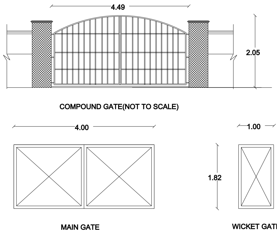
MAIN GATE
