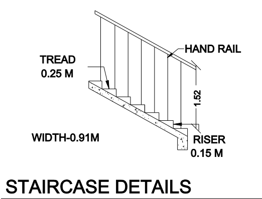
STAIRCASE DETAILS
