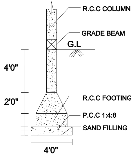
COLOUMN FOUNDATION
