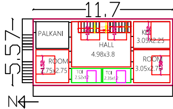
FIRST FLOOR PLAN & TERRACE FLOOR PLAN
