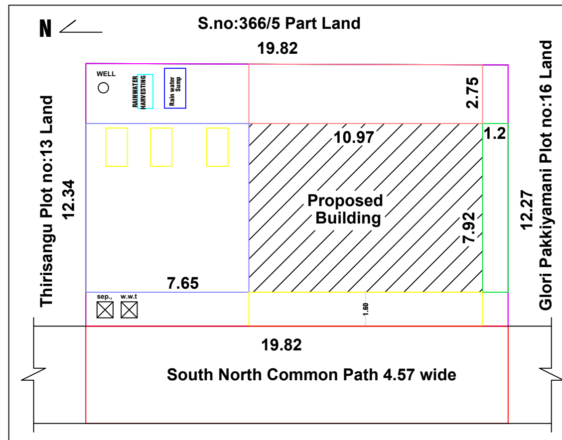
SITE PLAN CUM KEYPLAN
