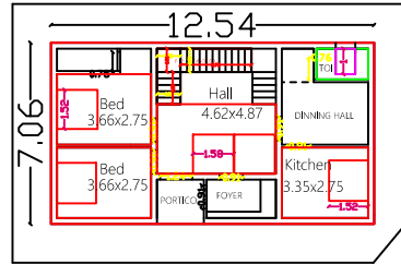
SITE PLAN CUM GROUND FLOOR PLAN
