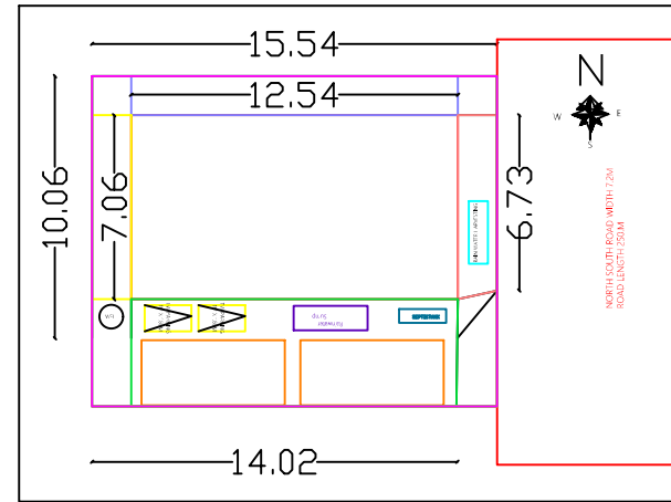
SITE PLAN CUM GROUND FLOOR PLAN
