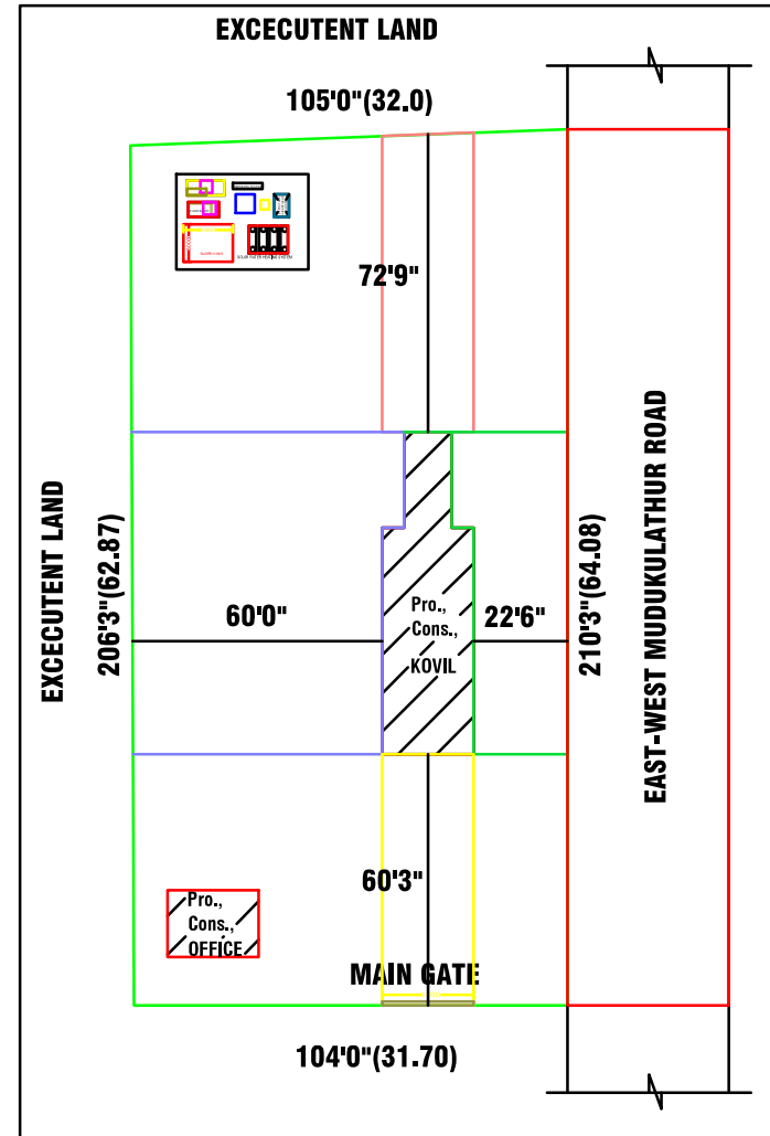
SITE PLAN
