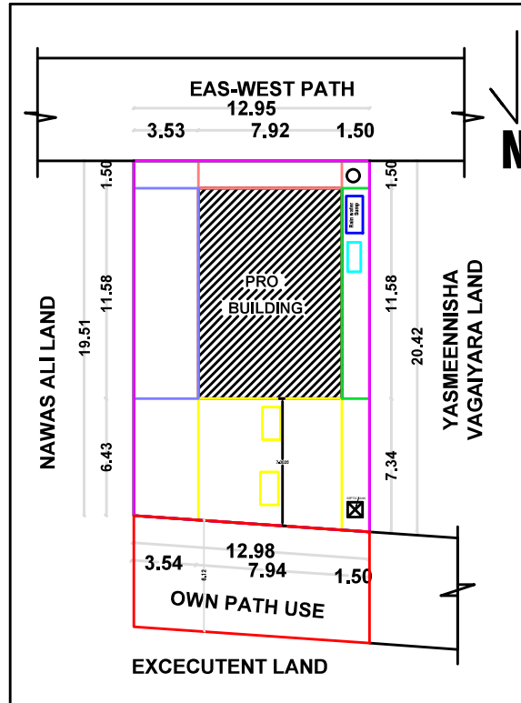
SITE PLAN & KEY PLAN
