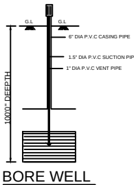
BORE WELL
