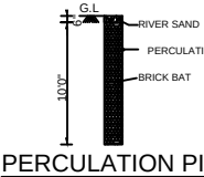
PERCOLATION PIT
