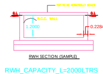
RW SECTION (SAMPLE) RW_CAPACITY_L=2000LTRS
