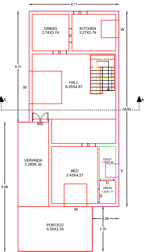
PROPOSED RESIDENTIAL GROUND FLOOR PLAN
