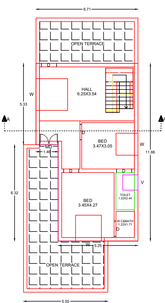
PROPOSED RESIDENTIAL FIRST FLOOR PLAN
