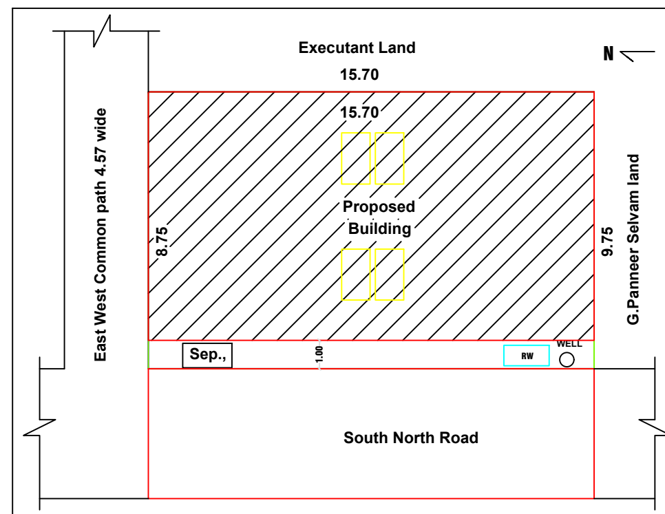
SITE PLAN CUM KEYPLAN
