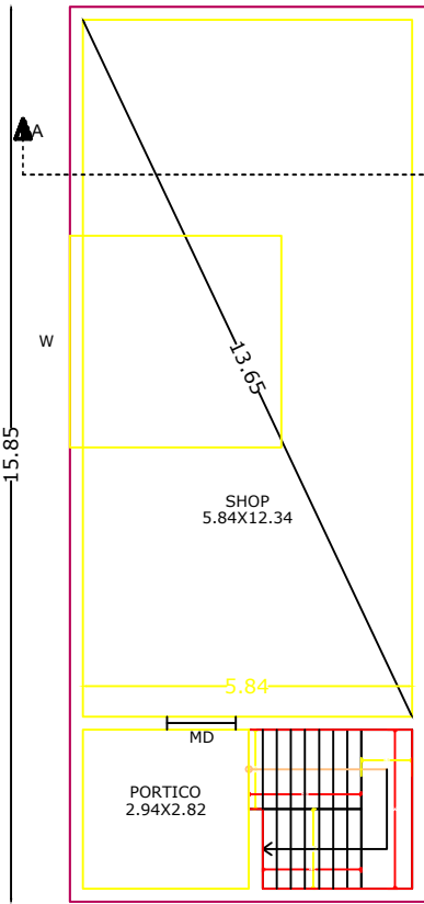
EXISTING COMMERCIAL GROUND FLOOR PLAN
