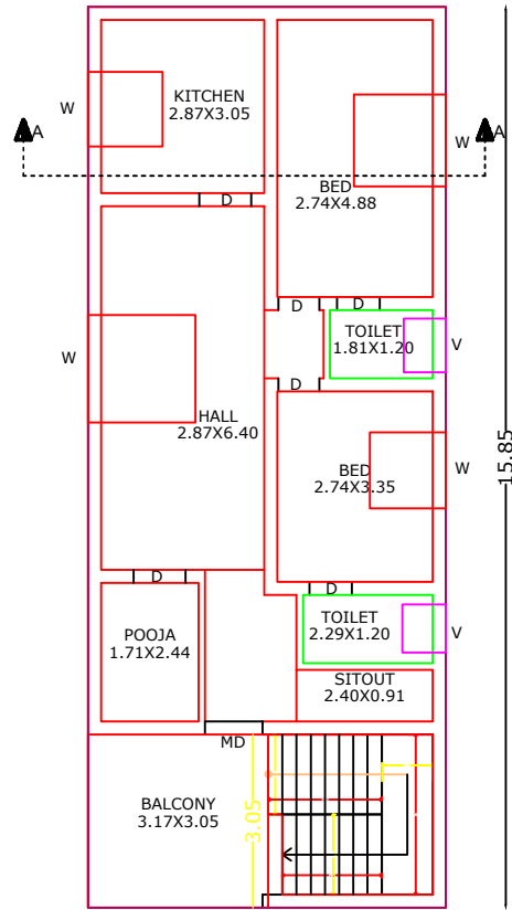
PROPOSED RESIDENTIAL FIRST FLOOR PLAN
