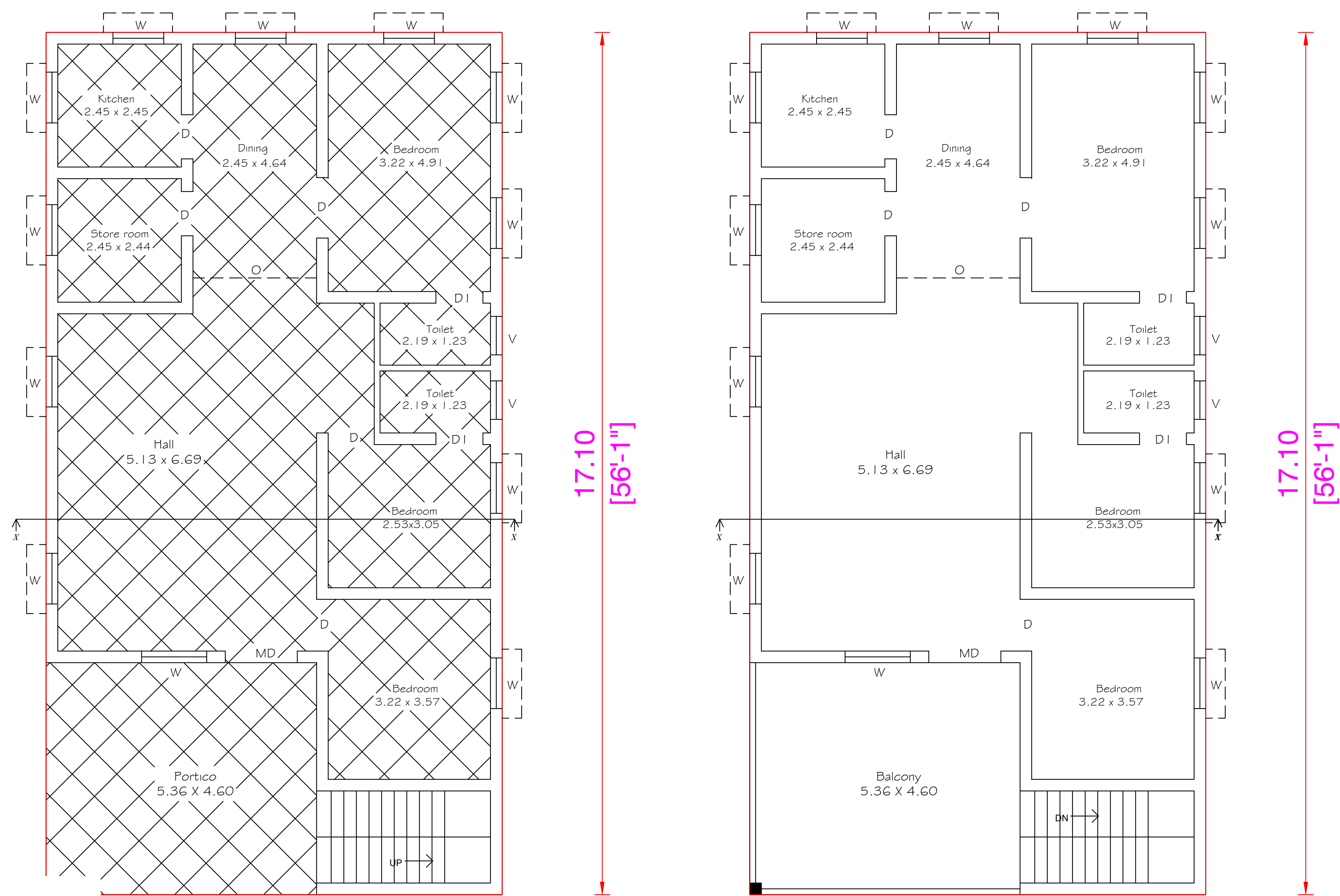
EXISTING GROUND FLOOR PLAN Ground floor B.A.No:1/2023-2024
