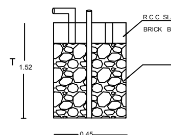
RAIN WATER STORAGE
