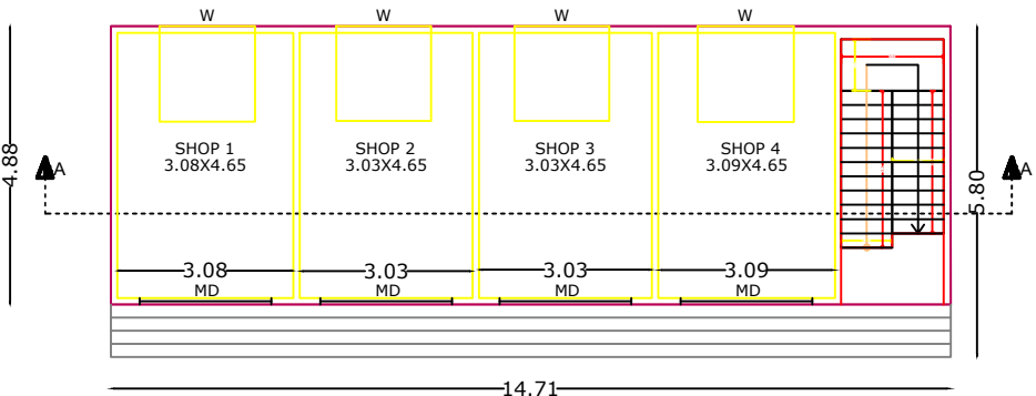
PROPOSED COMMERCIAL GROUND FLOOR PLAN
