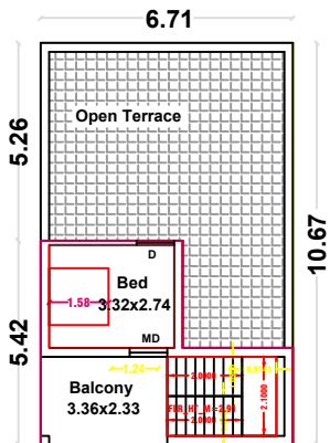
PROPOSED SECOND FLOOR PLAN
