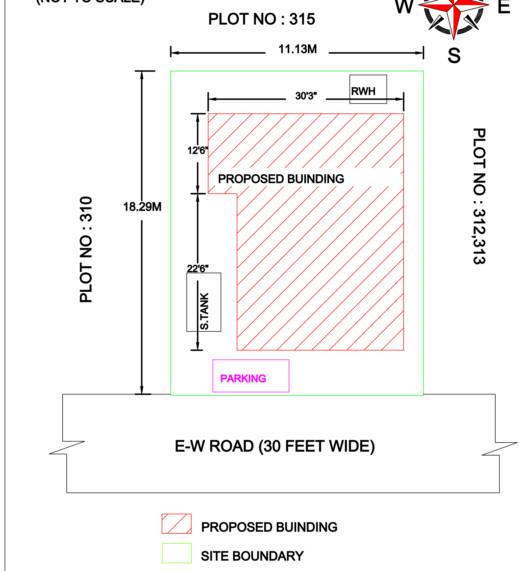
SITE PLAN
