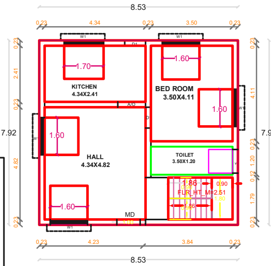
GROUND FLOOR PLAN PROPOSED
