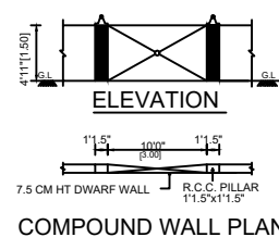
COMPOUND WALL PLAN
