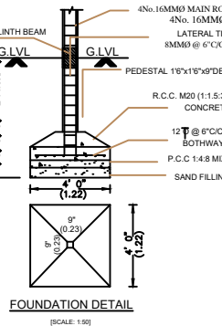
FOUNDATION DETAIL
