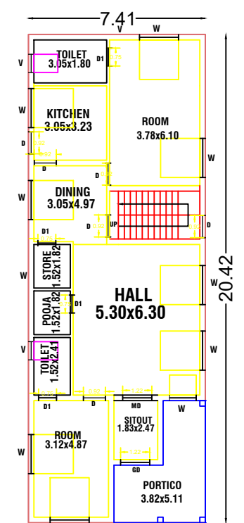
PRO., GROUND FLOOR PLAN
