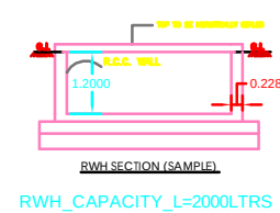
RWH_SECTION (SAMPLE) RWH_CAPACITY_L=2000LTRS
