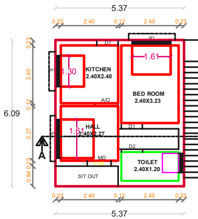
GROUND FLOOR PLAN PROPOSED
