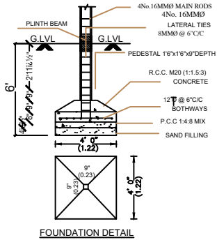
FOUNDATION DETAIL
